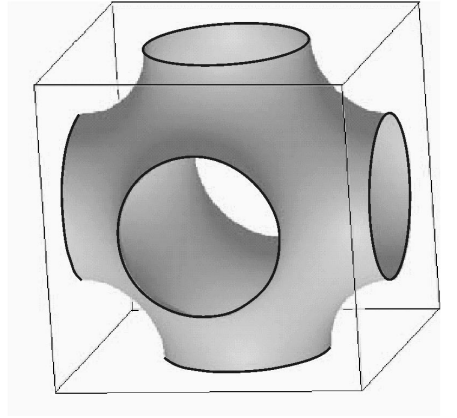
FIGURE 1. P Schwarz minimal surface is conjectured to have least area among surfaces dividing the 3-space into two Pm\bar{3}m -invariant regions with equal volume fractions.
